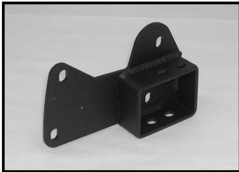
R403 / Qty. 1 Driver side radius arm relocation bracket
