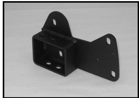
R404 / Qty. 1 Passenger side radius arm relocation bracket
