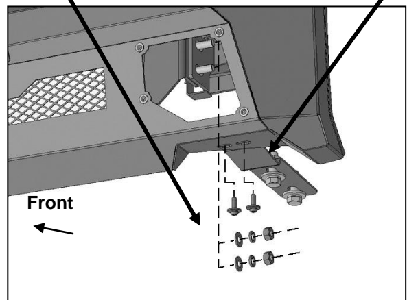
(Fig 18) Attach driver/left side of Bumper to Double Bolt Plate. Attach bottom of Bumper to Support Bracket
